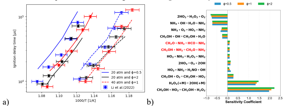
Figure 1. a) RCM experiment with 20/80 \text{CH}_3\text{OH}/\text{NH}_3 mixture at intermediate temperature. b) Sensitivity analysis on OH radical at 900 K and 20 bar.
