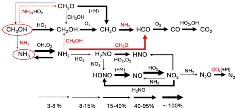
Figure 2. C ( \text{CH}_3\text{OH} ) and N ( \text{NH}_3 ) flux analysis at 1% \text{CH}_3\text{OH} conversion.
